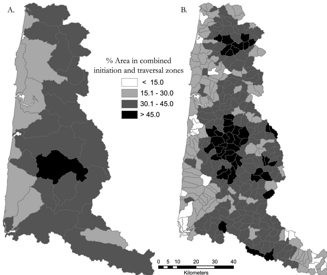
Figure 6. Spatial variation across the study area in the distribution of initiation and traversal zones for the combined 75% alternative. The percent of basin area encompassed by the alternative summarized by (A) 5th-field HUs and (B) in 7th-field HUs.
