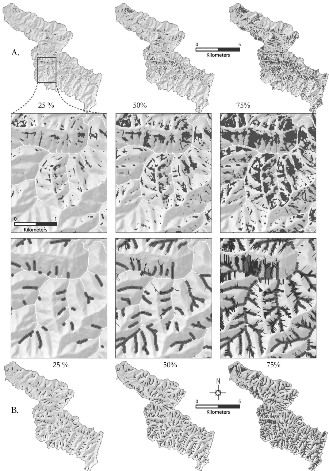
Figure 5. Initiation and traversal zones illustrated for the Knowles Creek basin. The modeled fish-bearing channel network is shown in white. (A) Initiation zones are in dark gray and include 25%, 50%, and 75% of initiation sites for landslides that delivered to fish-bearing channels. (B) Traversal zones are in black and include 25%, 50%, and 75% of pixels traversed by debris flows that delivered to fish-bearing channels. Gray polygons include 35-m extensions for traversal zones along all nonfish-bearing streams.
