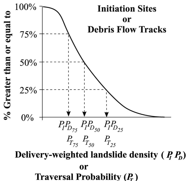
Figure 3. A sketch illustrating the threshold probabilities necessary to include different percentages of initiation or traversed pixels. Probabilities are of initiating ( P_I P_D ) a landslide that delivers to a fish-bearing channel or of being traversed ( P_T ) by a debris flow that delivers to a fish-bearing channel.
