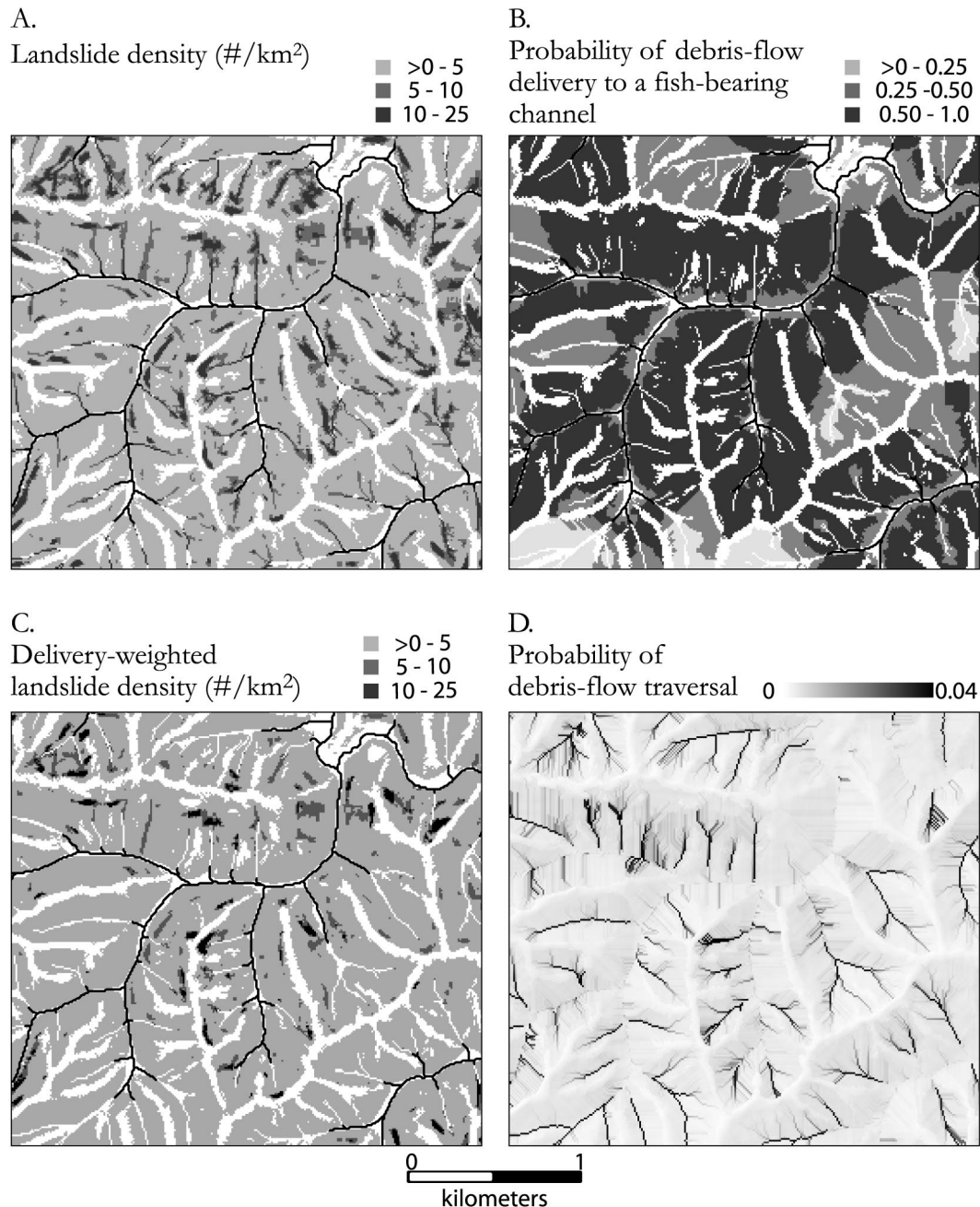
Figure 2. Outputs of the coupled debris-flow initiation and delivery model (Miller and Burnett 2007; Miller and Burnett in review) illustrated for a portion of the Knowles Creek basin in the central Oregon Coastal Province, USA. (A) Modeled landslide density. (B) Probability of debris-flow delivery to a fish-bearing channel. (C) Delivery-weighted landslide density expressed for each pixel as the product of the landslide density and the probability of debris-flow delivery to a fish-bearing channel. (D) Probability that a pixel is traversed by a debris flow that traveled to a fish-bearing channel. This probability is presented over a hill-shade view of the underlying DEM.
