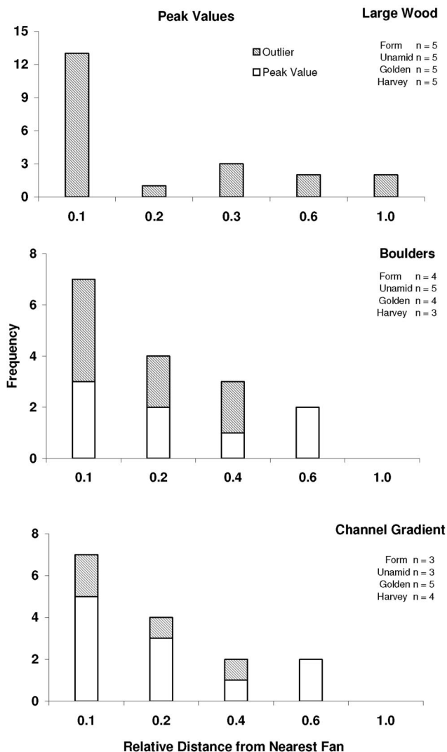
Figure 5. Frequency histograms of peak channel parameters by relative distance from nearest fan showing higher peak values near fans. The proportion of peak values that are also outliers is shown by hatch marks. To normalize the reach distances from nearest fan across the four study sections, the reach distances from fan were divided by the longest reach distance from fan within each of the four study sections (see Methods section), resulting in a relative distance from nearest fan for the x axis. While thicker wedges of sediment are often associated with increased boulder accumulations at fans, they also extended upstream and downstream from debris fans (Figure 7, Appendix C), and consequently were not detected in our peak value analysis and therefore not shown here.
