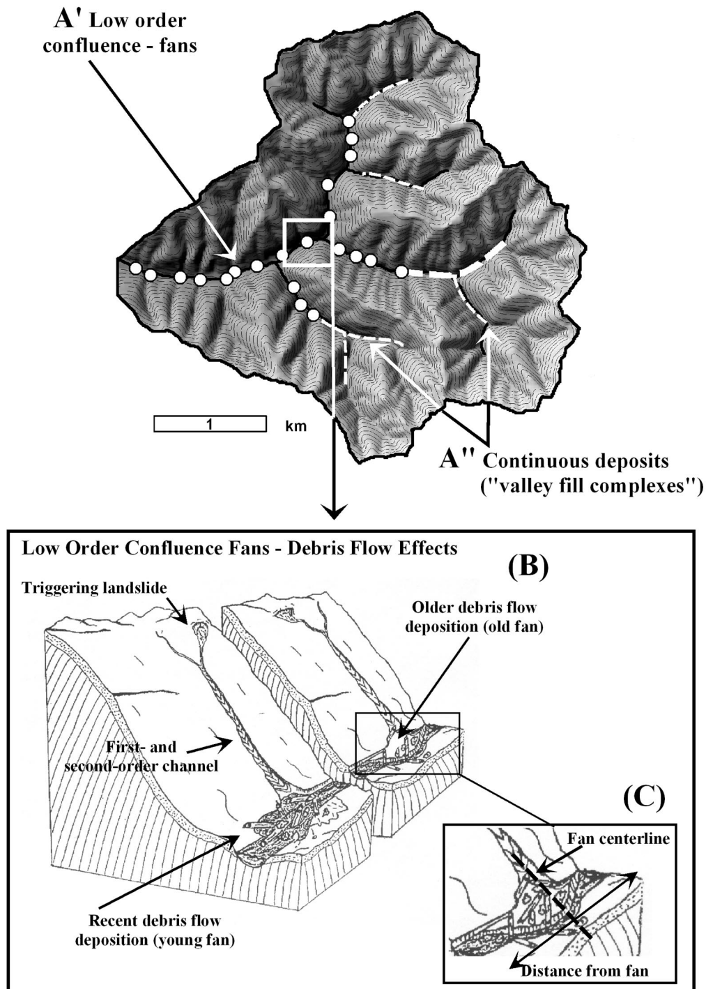
Figure 2. (A) Patterns of debris flow deposition in Harvey Creek basin. (A') White dots represent observed debris flow deposits (debris fans) at confluences of first- and second-order headwater streams observed in the field and predicted using the model of Benda and Cundy (1990). (A'') Dashed white lines show colluvial valley fill complexes where debris flows create semicontinuous deposits and terraces along upper third-order channels as modeled by Benda and Dunne (1997). (B) Effects of deposits depend, in part, on their age. (C) Morphological effects of debris flows were evaluated according to the distance from nearest (upstream or downstream) "fan centerline."
